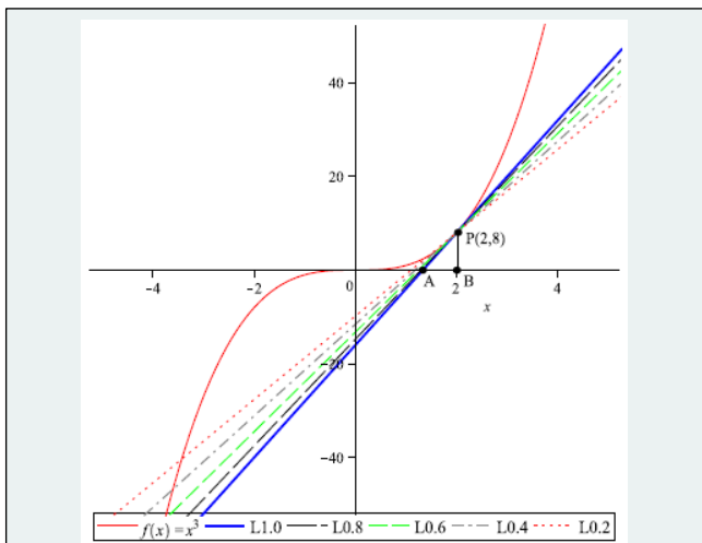
FIGURE 3. GRAPH OF THE FUNCTION F(X) = X^3 WITH TRIANGLES FORMED WITH FRACTIONAL ORDER DERIVATIVES [15].
